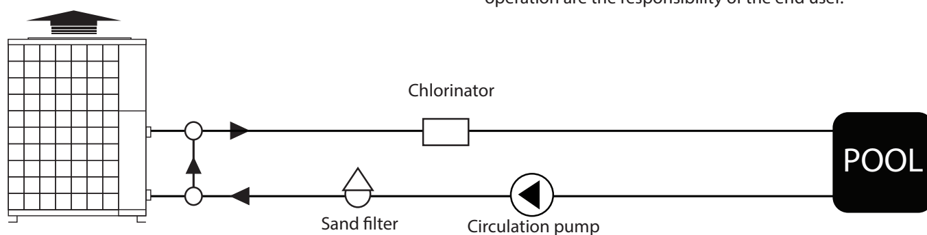
Outline diagram for installation of X-series
